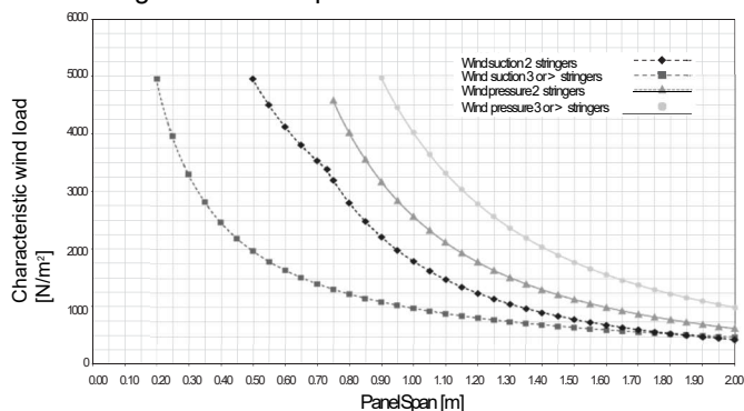
Design chart of 150F panel
