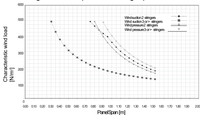
Design chart of 70U panel with locking clip
