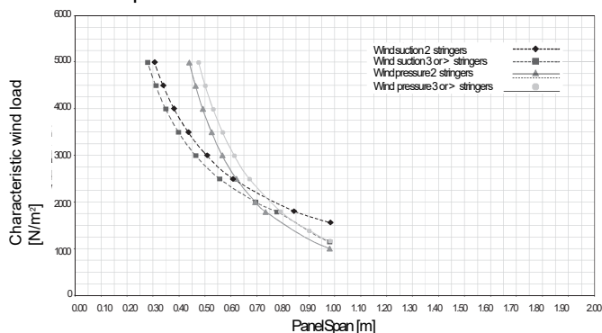
Panel spans 150C
