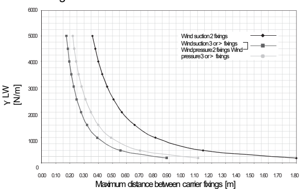
Design chart of carrier 150F
