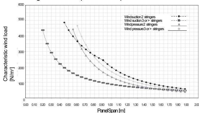
Design chart of 80B panel with clip
