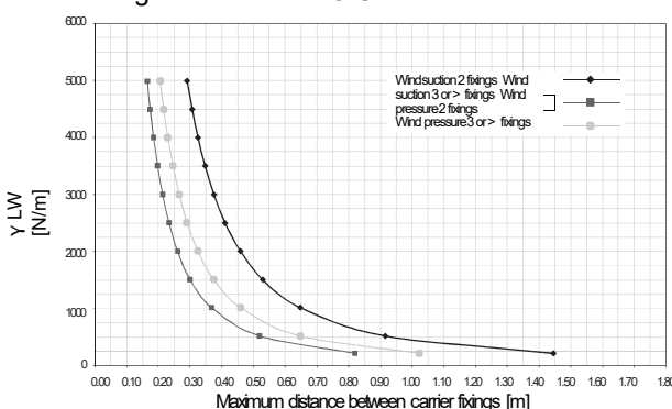
Design chart of carrier 84C
