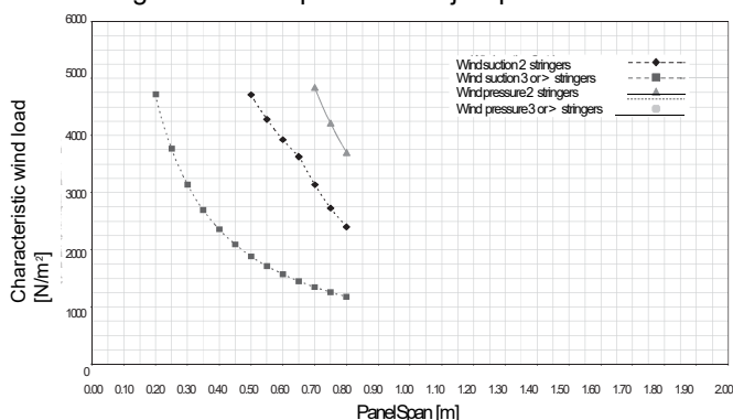
Design chart of 84R panel with V5-join profile
