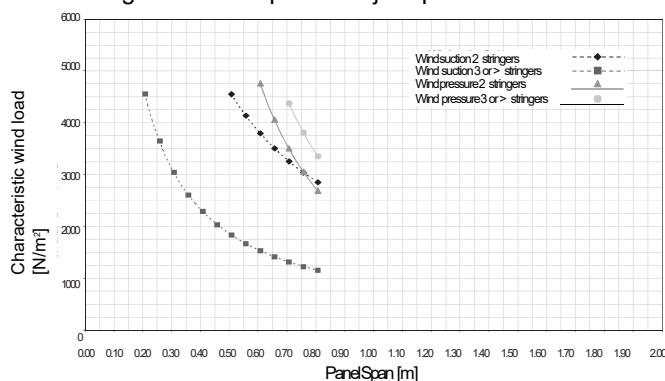
Design chart of 80B panel with join profile
