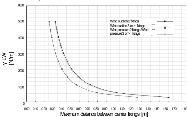
Design chart of carrier 80B
