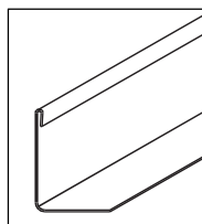
Wall L-profile Alu (45 x 32.5)
