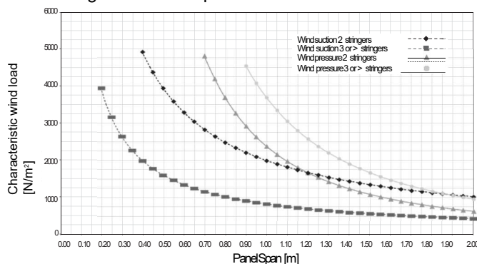
Design chart of 200F panel
