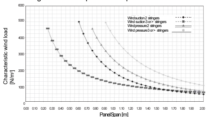
Design chart of 150F panel with clip
