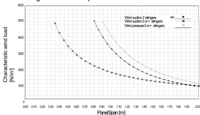
Design chart for 185U panel
