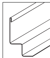
Wall W-profile Alu (45 x 21 x 21 x 18.5)
