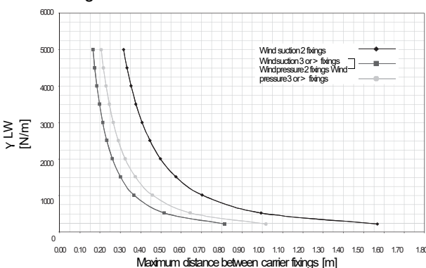
Design chart of carrier 84R
