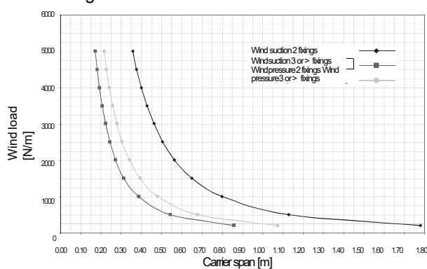
Design chart of carrier 200F
