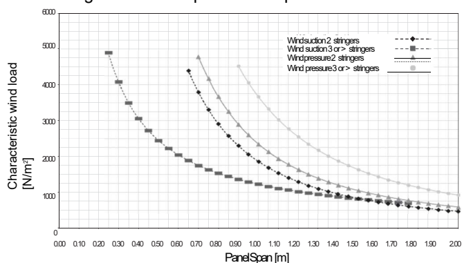
Design chart of 200F panel with clip
