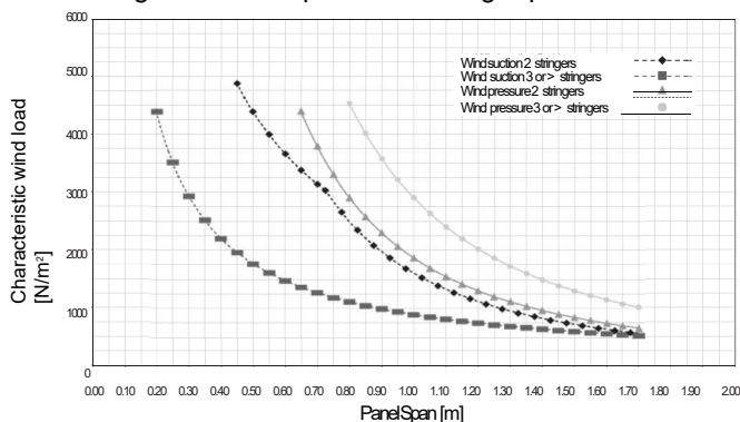
Design chart of 84R panel with locking clip
