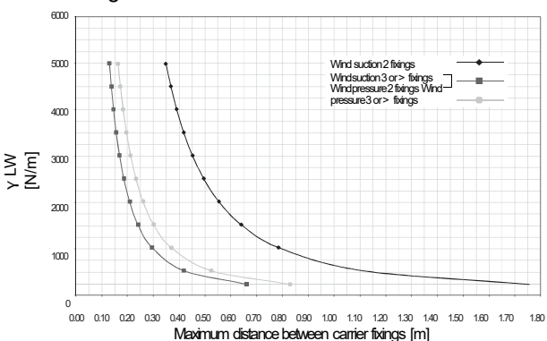
Design chart of carrier 185U
