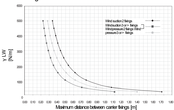
Design chart of carrier 84B
