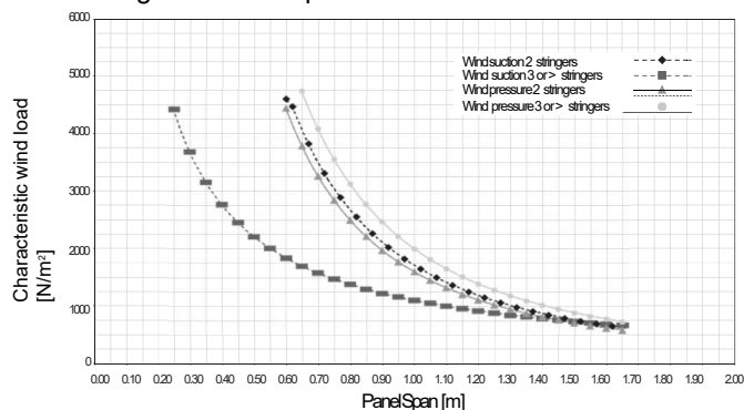
Design chart of 84B panel
