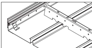
Mounted system
