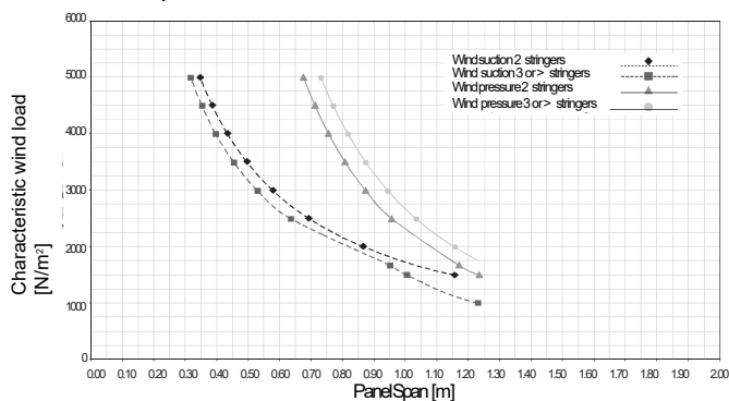
Panel spans 75C
