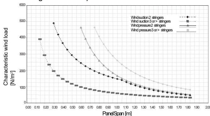
Design chart of 84C panel
