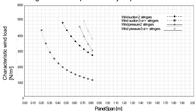
Design chart of 84R panel with U-join profile
