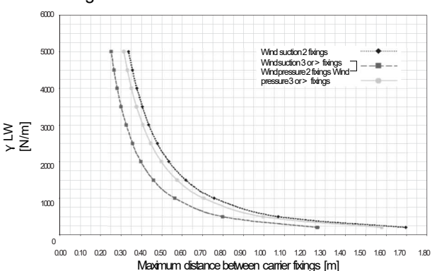
Design chart of carrier 70U
