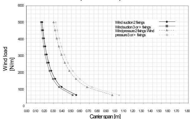
75C-225C Carrier spans closed panels
